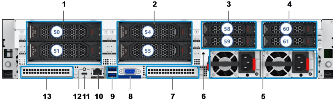
Figure 2-11 Sabit Diskli Arka Panel
